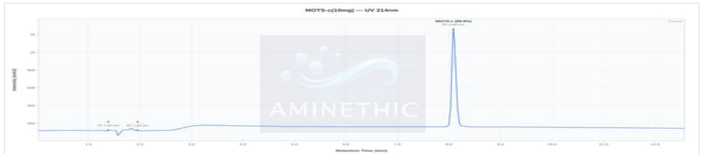
MOTS-C 10mg - MTC0003 : UV Chromatogram
